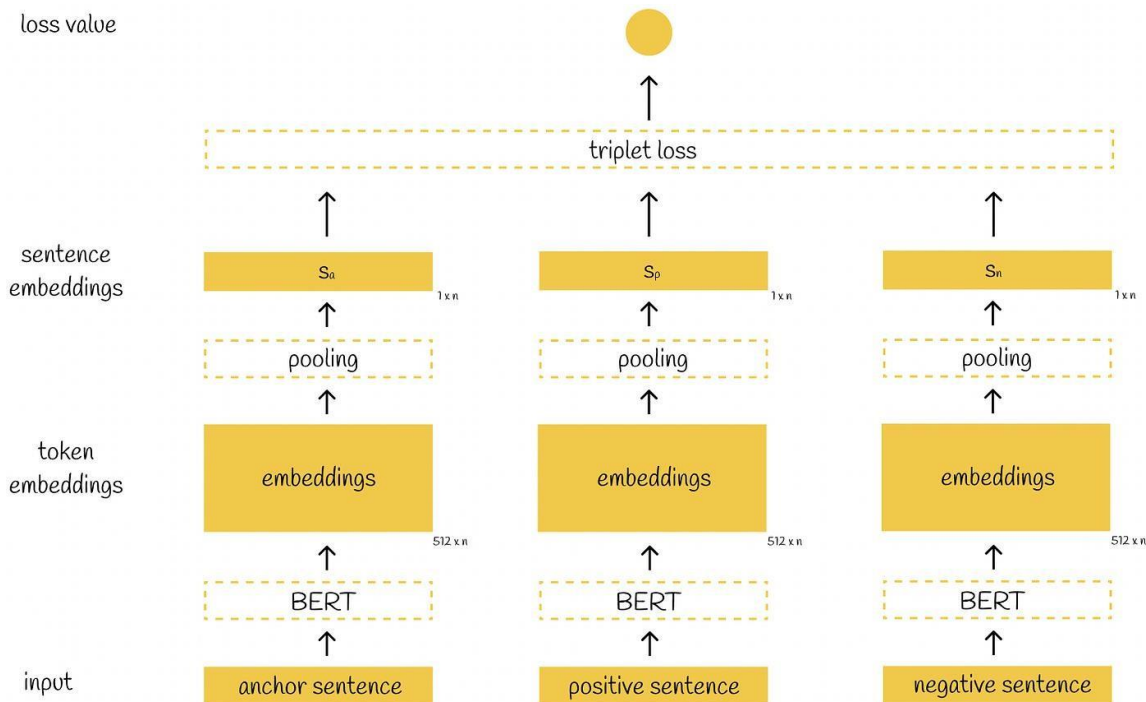
Figure 5.1.1: Sentence-BERT Diagram
